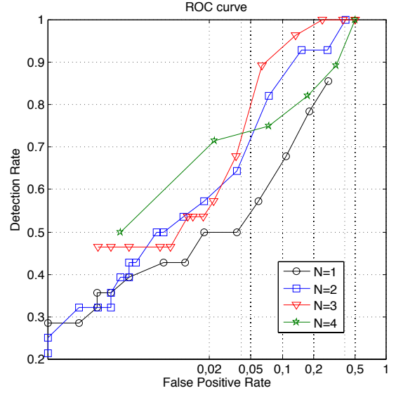
Fig. 3. ROC curves resulting from KL expansion to the dataset with only mean removal for different value of the temporal correlation range.
