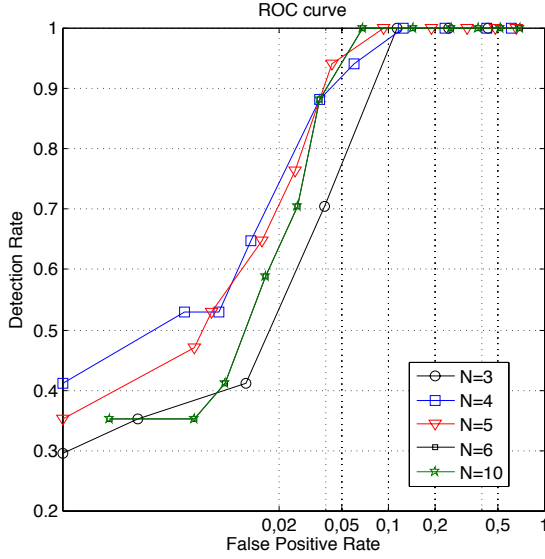
Fig. 5. ROC curves obtained over the first week of data for different values of N .
