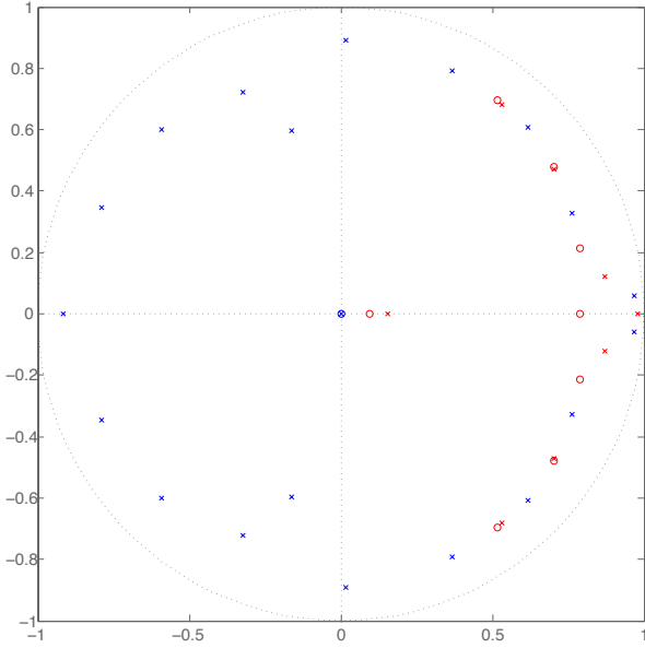
Fig. 8. Pole-zero diagrams of the initial system (in blue) along with the predictive model with 8 components (in red).
