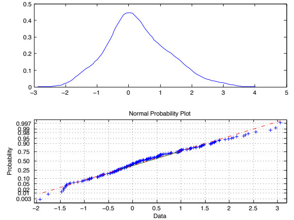
Fig. 4. Normal plot of normalized decision variable D[k] for N = 3
