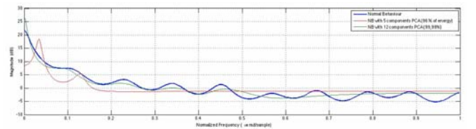
Fig. 7. Spectra of the initial signal compared with the signal resulting from the predictive models using KL expansion with an increasing number of components.
