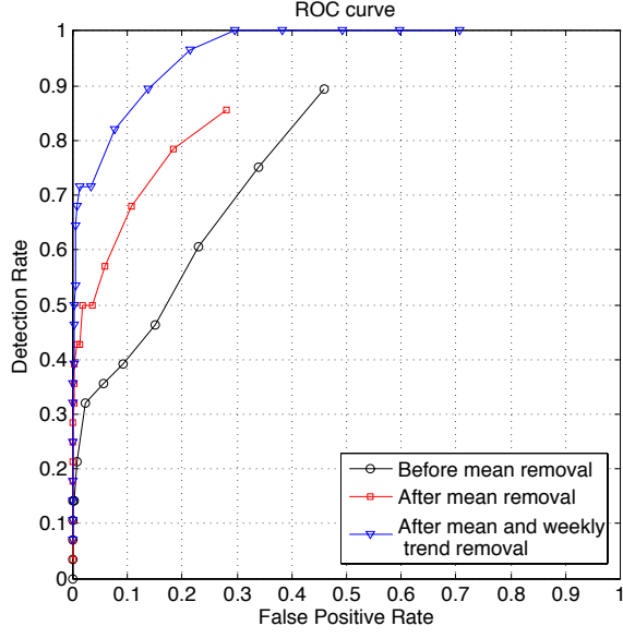
Fig. 1. ROC curve resulting from application of PCA method to three variation of traffic metrics.
