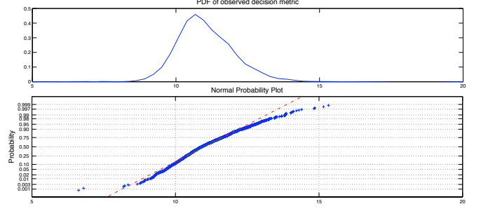
Fig. 2. Normal plot of normalized decision variable D[k] for UDP traffic obtaining over the data used for calibrating the PCA model
